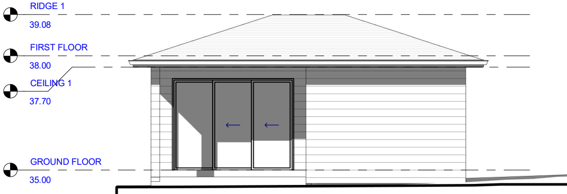
5 SOUTH-WEST ELEVATION_NP DA.14 1 : 100
